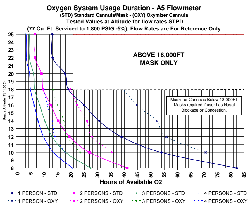
Figure 24 - A5 Flowmeter (Oxymizer and Standard Scales)
