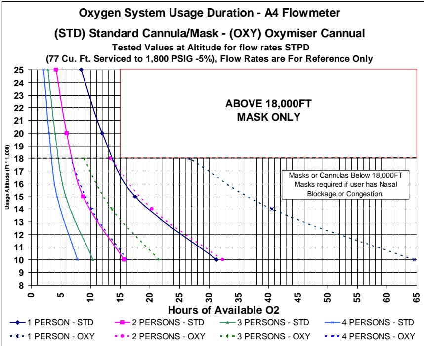
Figure 23 - A4 Flowmeter (Oxymizer and STD Scales)
