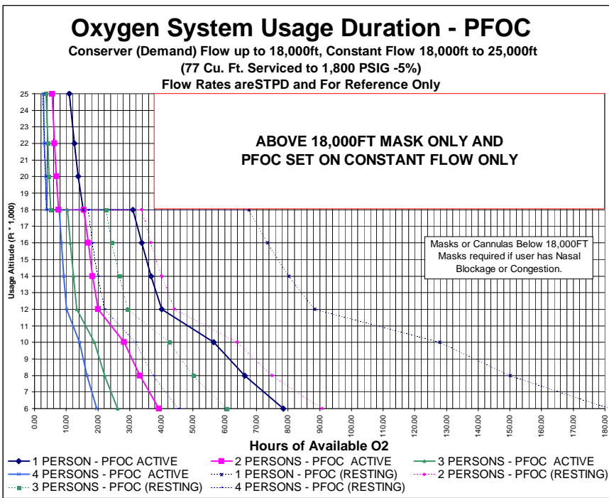
Figure 25 - PreciseFlow Oxygen Conservser
