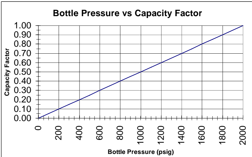
Figure 22 - Bottle Pressure/Capacity Factor Graph
