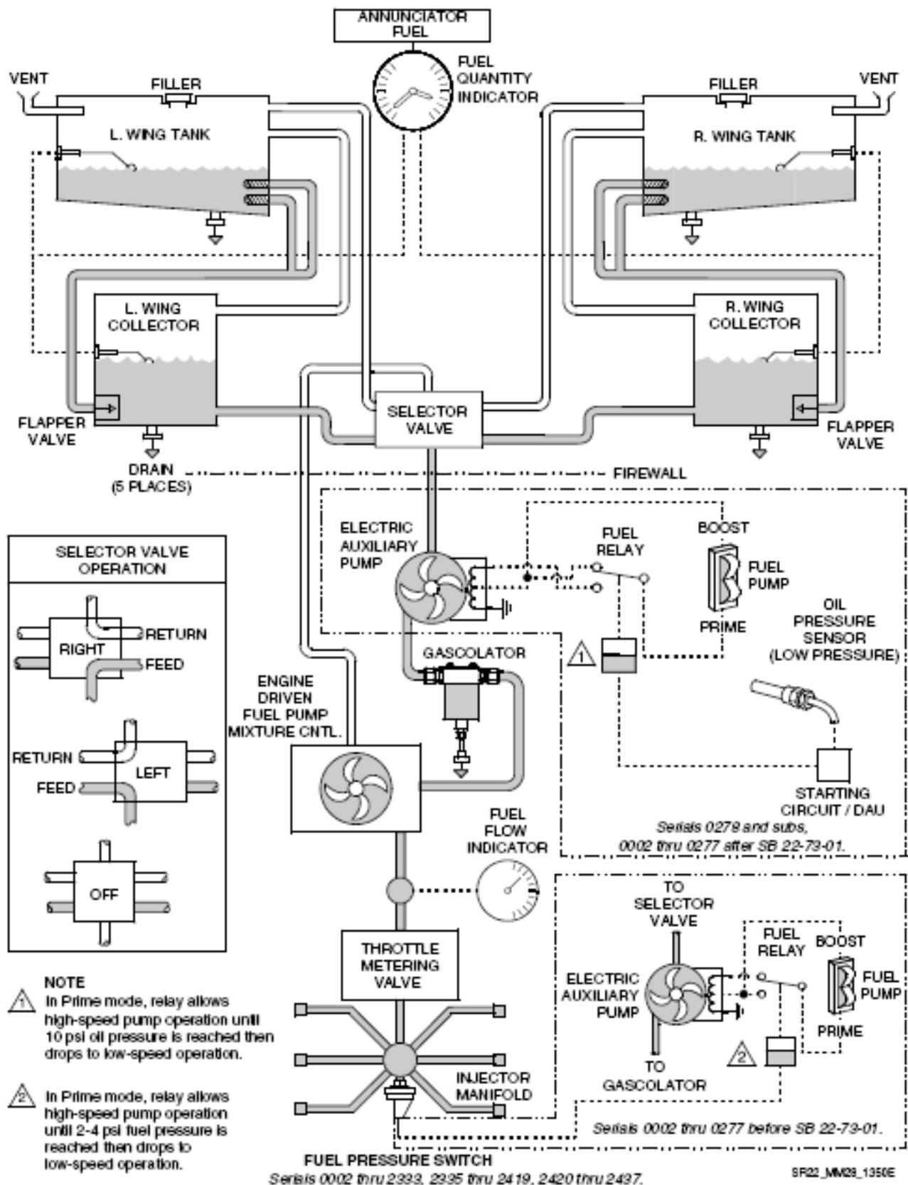
Figure 28-002 Fuel System Schematic - Serials 0002 thru 2437 (Sheet 1 of 2)
