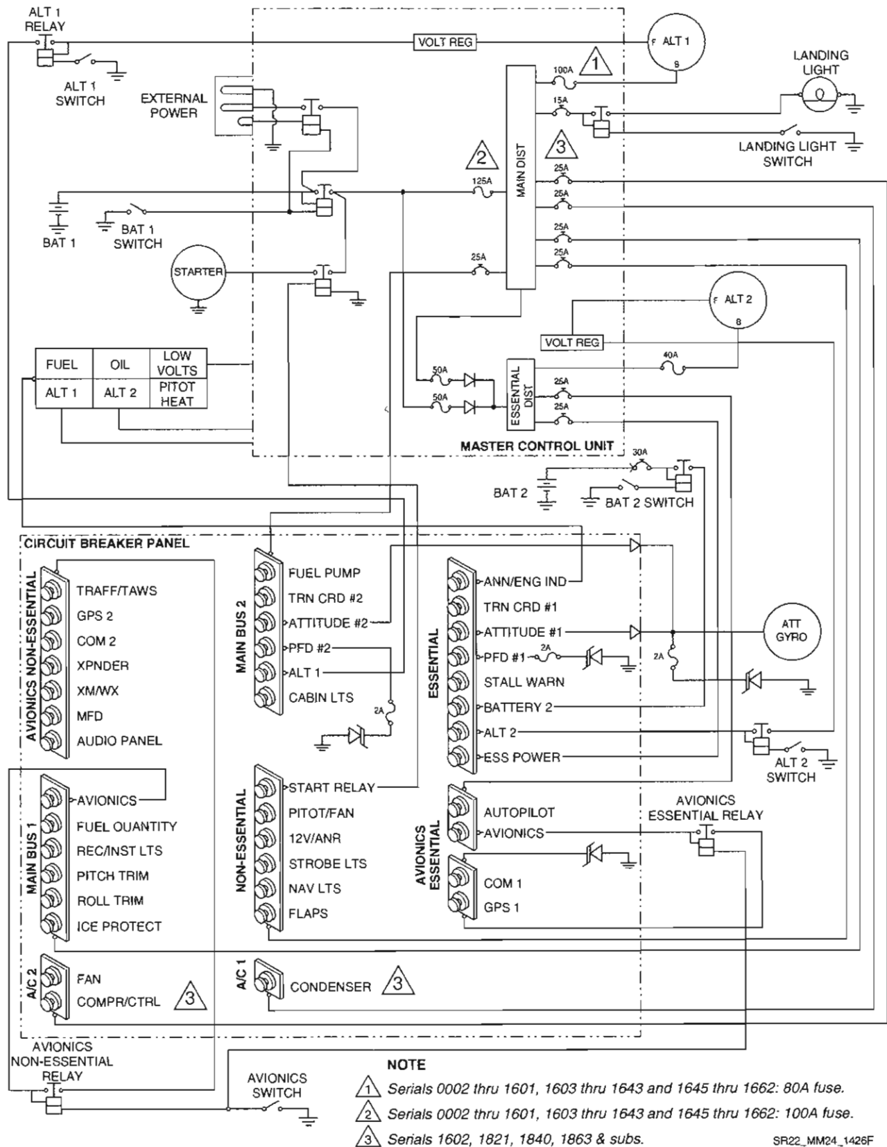
Figure 24-301 Electrical System Schematic - Serials 0002 thru 3025, 3026 & subs w/o Perspective Avionics
